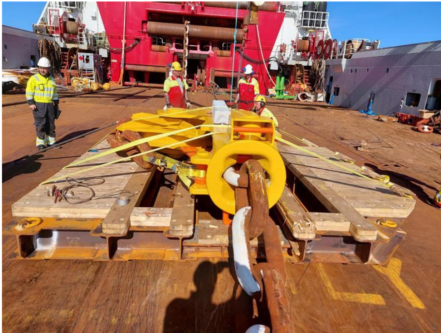
Inline tensioner skidding frame, designed by SEMAR.
