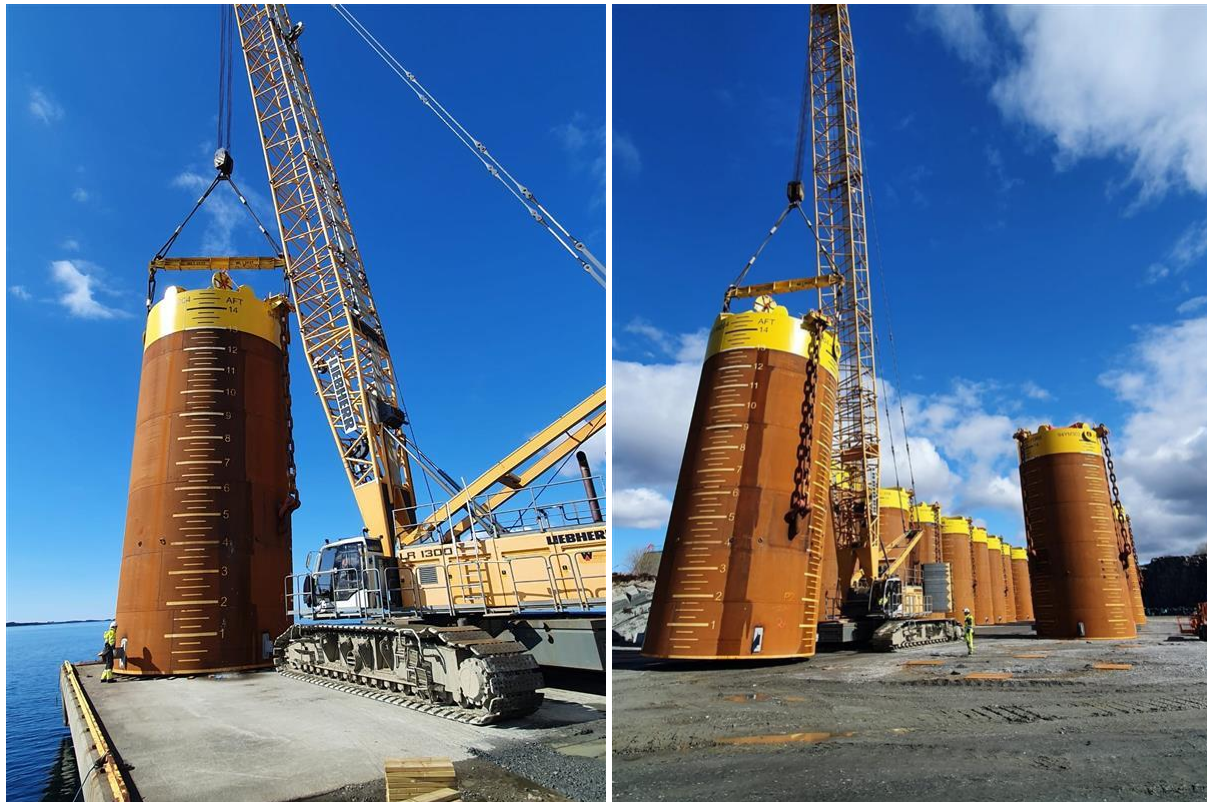
Equinor, Hywind Tampen - Suction anchors at key side. Ready for shipping to site
